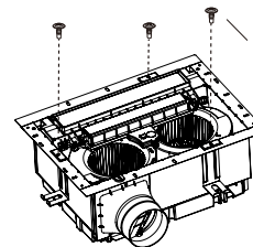
Self-tapping screws \phi 4 \times 13 自攻螺絲 \phi 4 \times 13
